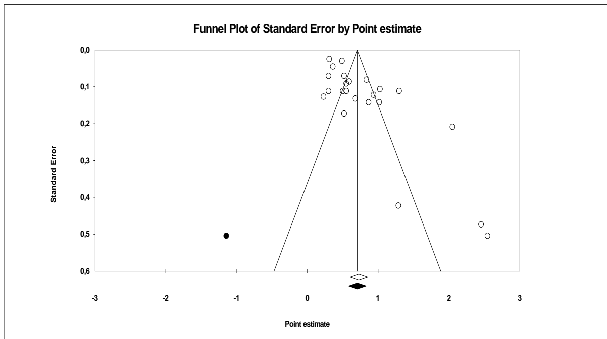
Figure 2. Funnel plot of the dataset
