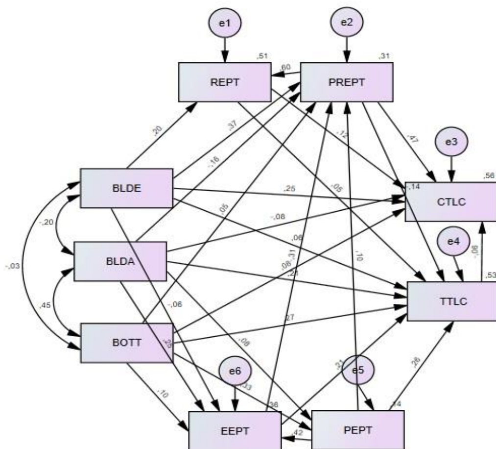
Figure 2. Standardized path coefficients
