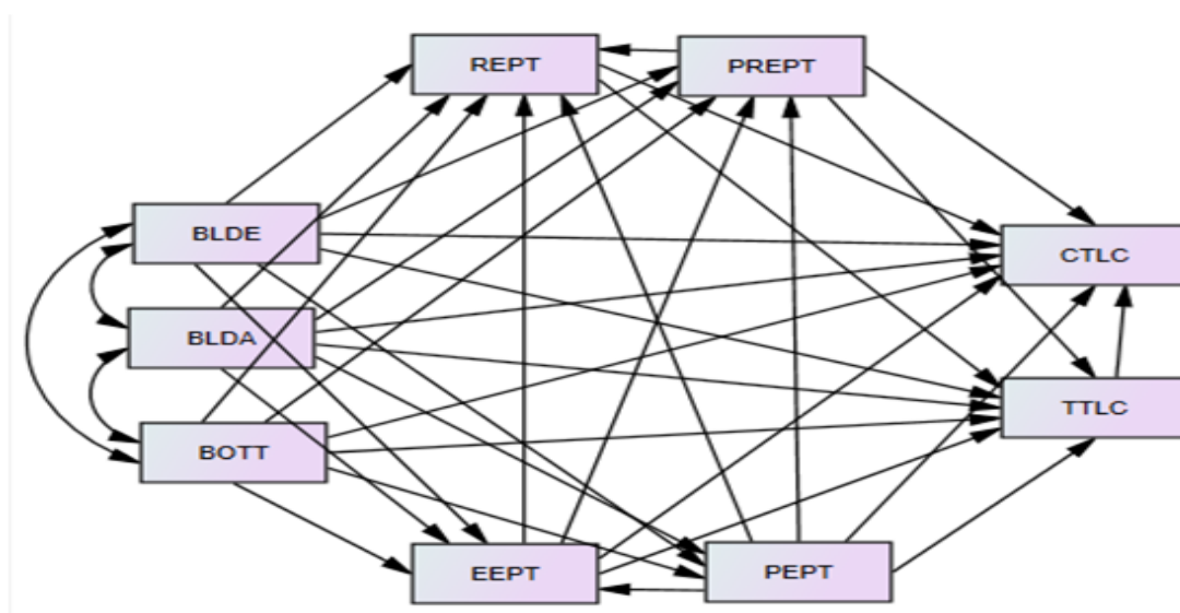
Figure 1. Theoretical model
